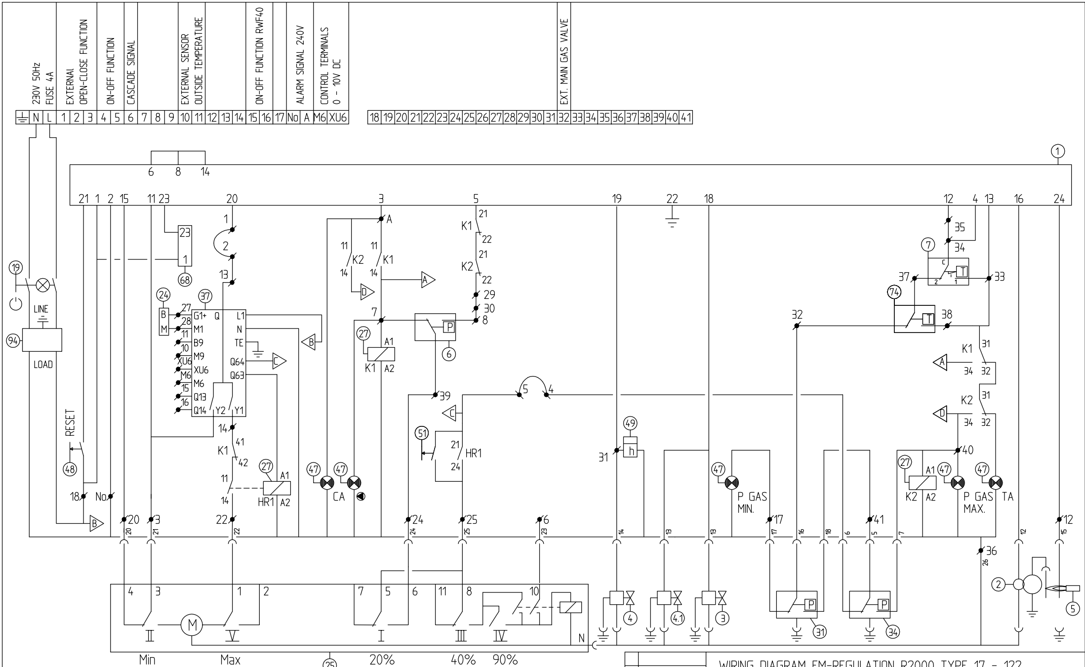
WIRING DIAGRAM EM-REGULATION R2000 TYPE 17 - 122 With fleu thermal cut out and min./max gaspressure.
